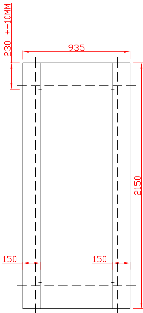
DOOR SIZE (STOCK) 935 X 2150 MM DOOR SIZE (CUT DOWN) 715 X 1750 MM
